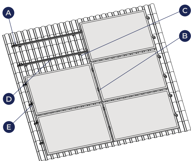
A BRIDE EXTER MODULE D RAIL
